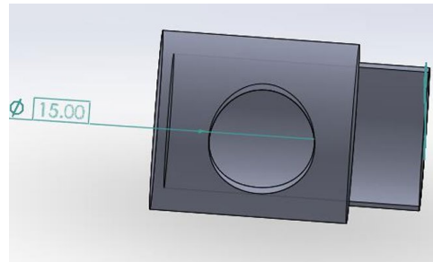
Figure 5. Nozzle design.
