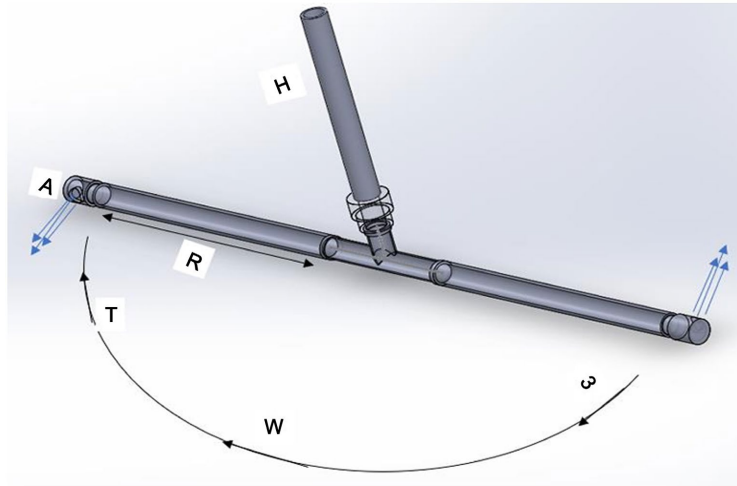
Figure 10. Rotor reference frame.
