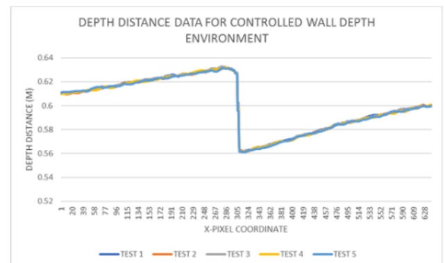
Figure 16 Depth Distance Data for Controlled Wall Depth Environment
