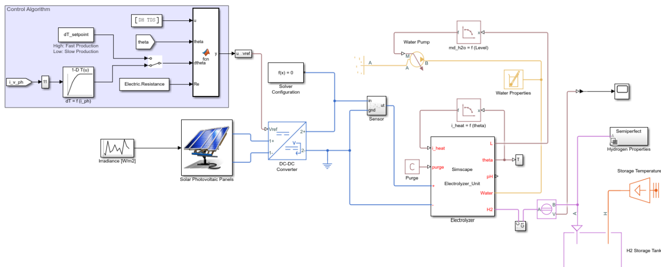
Figure 4 Simulation diagram [20]
