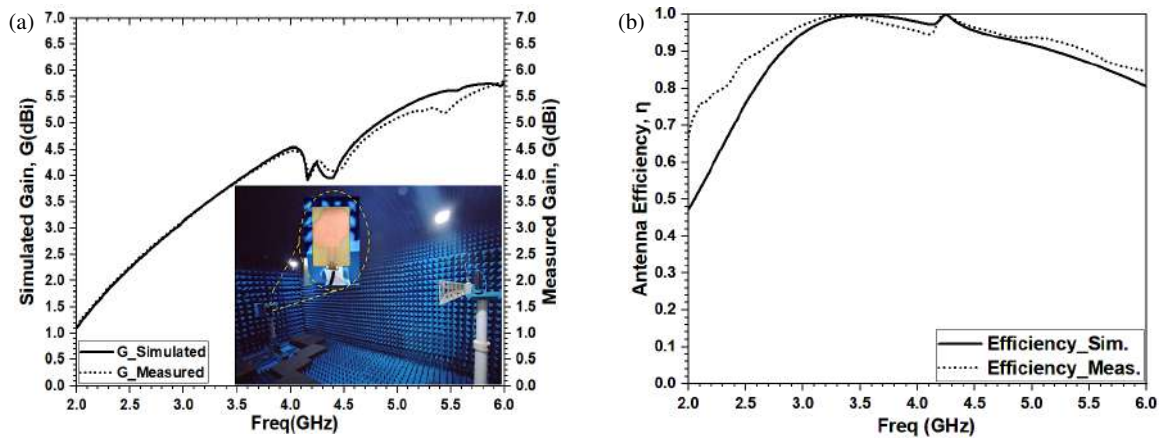
FIGURE 12. Simulated and measured (a) antenna gain, and (b) antenna efficiency.
