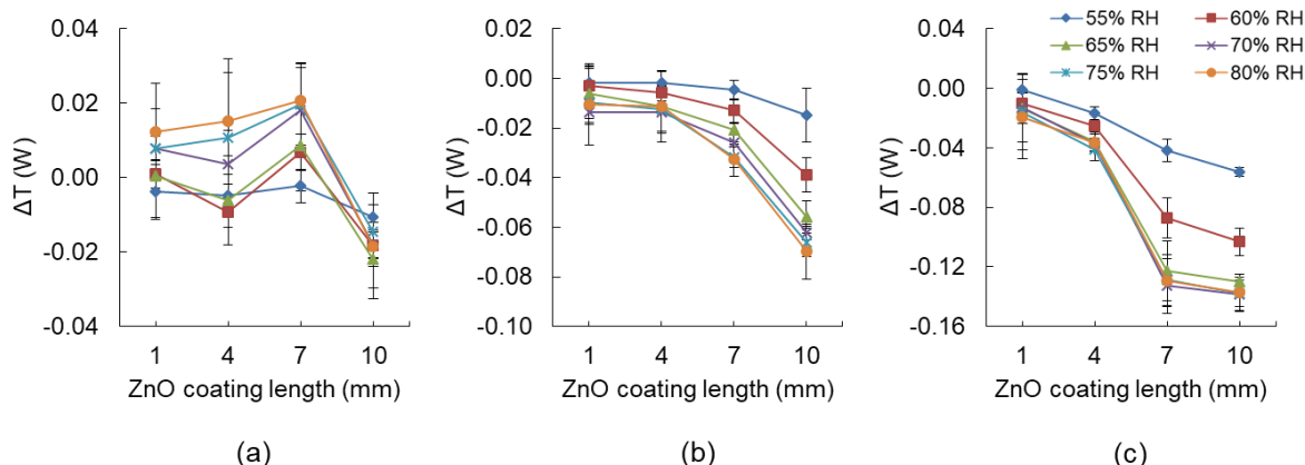
Figure 6: Humidity sensing response on ZnO coated glass substrates for the growth durations of (a) 5 h, (b) 10 h and (c) 15 h.
