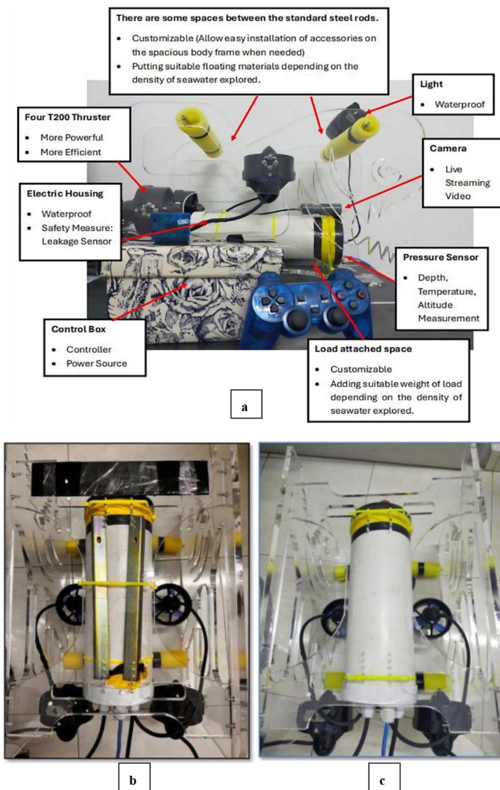
Figure 9. Components of designation ROV
