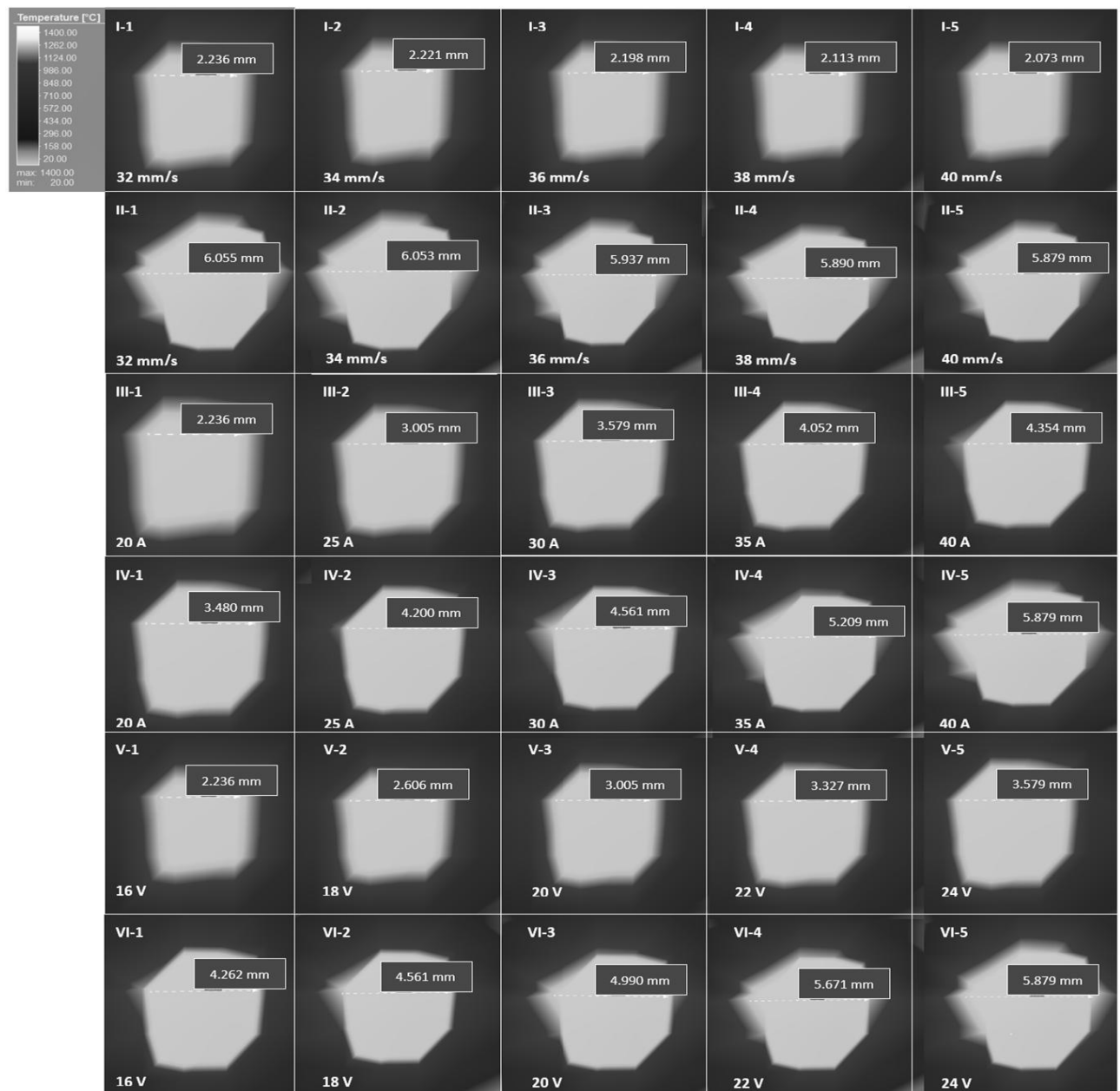
Fig. 4 WMP under different scan speeds (I, Current = 20A, Voltage = 16V) and (II, Current = 40A, Voltage = 24V), various current (III, Speed = 32mm/s, Voltage = 16V) and (IV, Speed = 40mm/s, Voltage = 24V) and at various voltage (V, Speed = 32mm/s, Current = 20A) and (VI, Speed = 40mm/s, Current = 40A)
