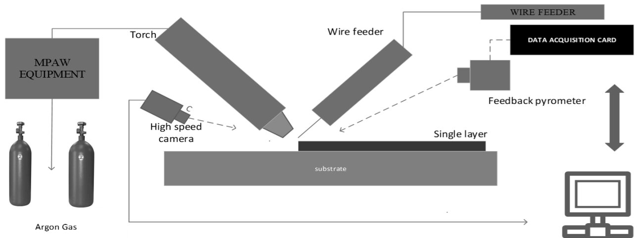
Fig. 3 Experimental Setup
