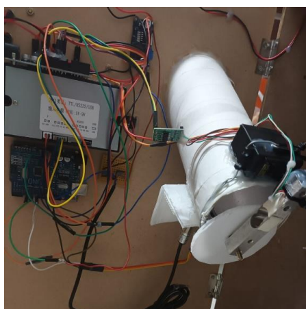
Figure 13: Hardware circuit inside MDD prototype
