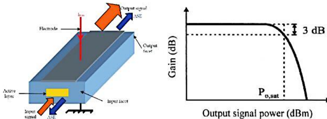
Fig. 1 SOA gain mechanism [62]
