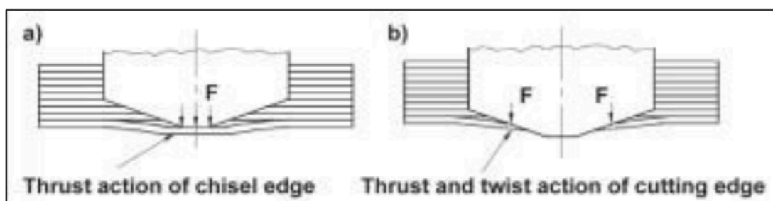
Figure 2.19: Development of Delamination (Sedlacek & Slany, 2019)
