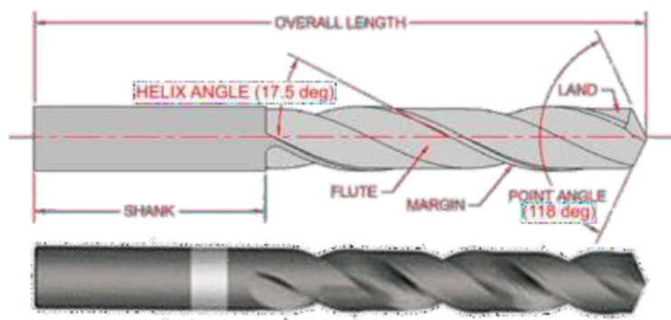
Figure 2.12: Twist Drill ( https://wiki.dtonline.org/index.php/Twist_Drills )
