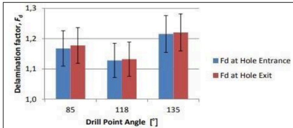
Figure 2.22: Drilling of 0.06 mm/rev of feed rate (Maoinsier et al., 2014)
