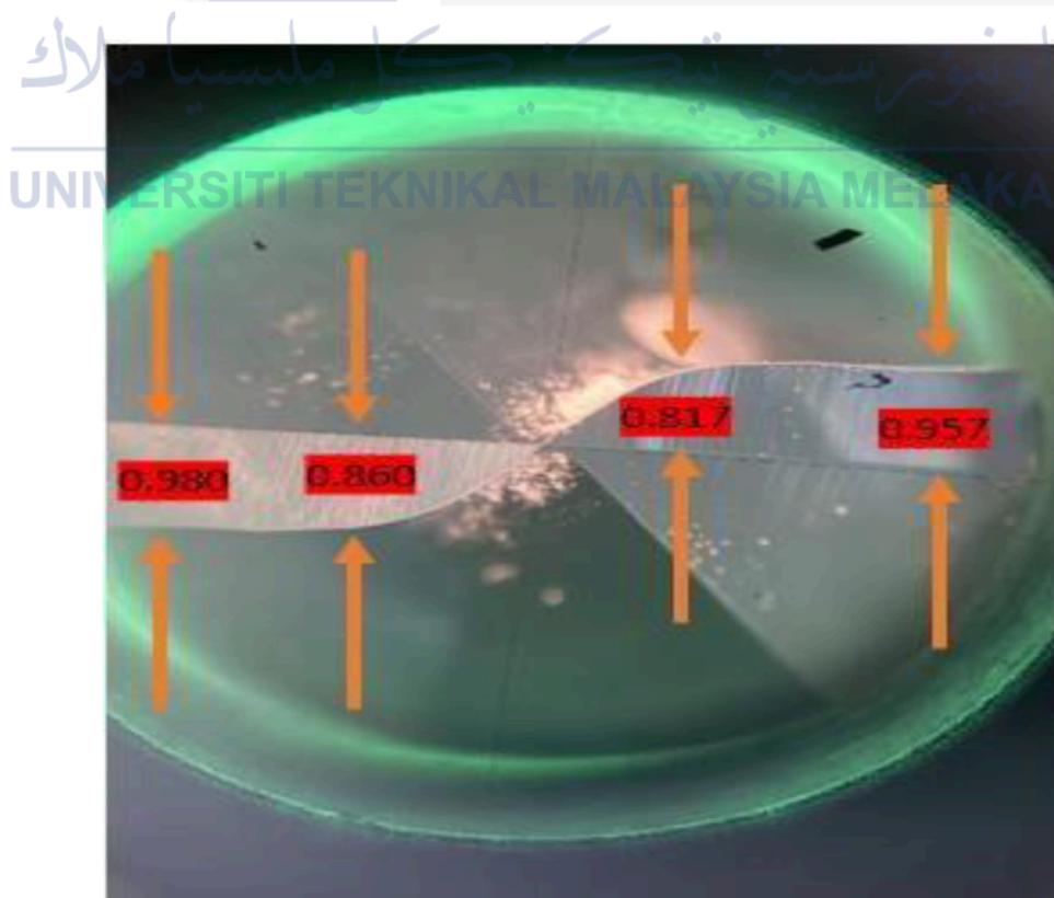
Figure 4.18: Flank Wear Measurements of Tool 6
