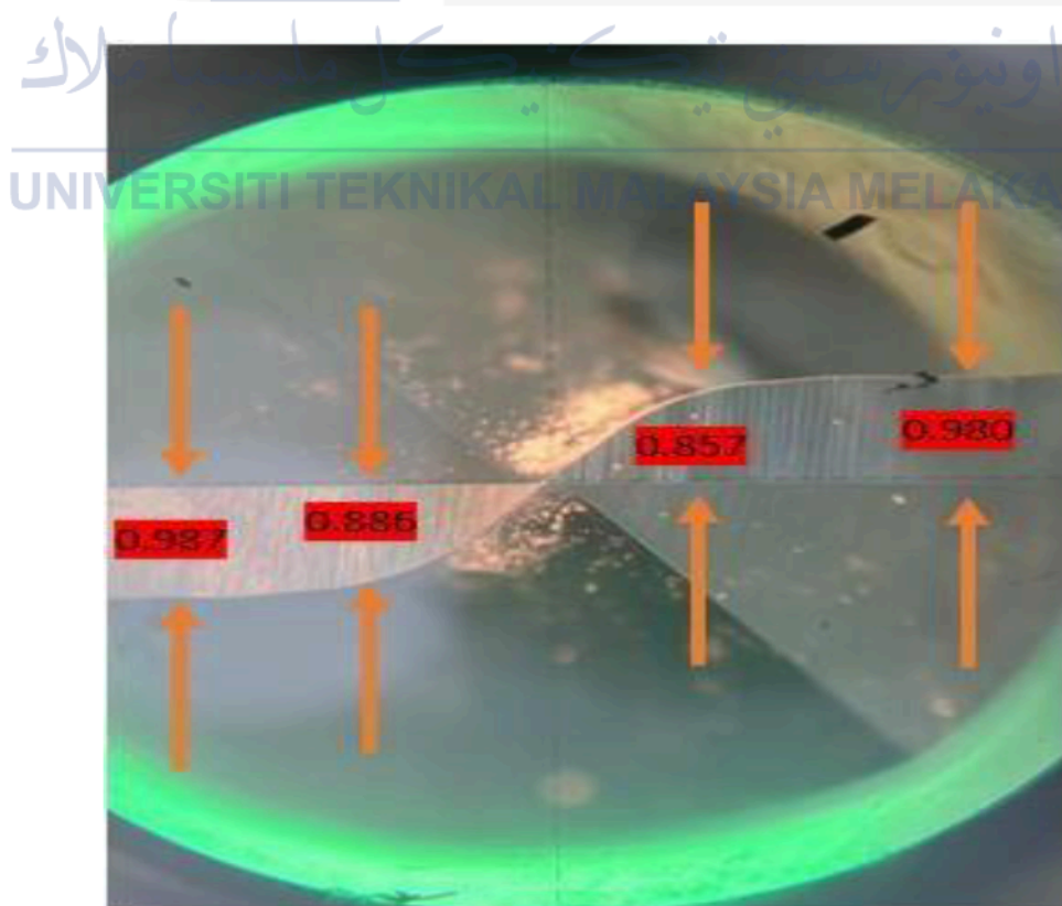
Figure 4.16: Flank Wear Measurements of Tool 4
