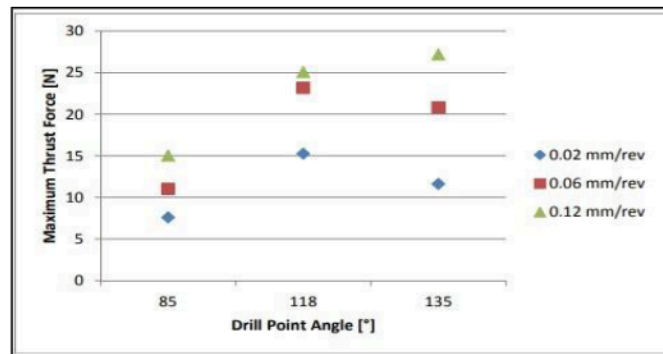
Figure 2.15: Effect of drill point angle on maximum thrust force. (Maoinsir et al., 2014)
