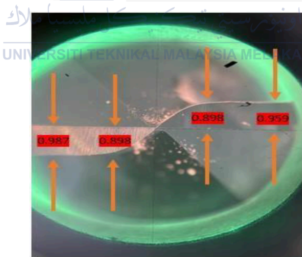
Figure 4.20: Flank Wear Measurements of Tool 8
