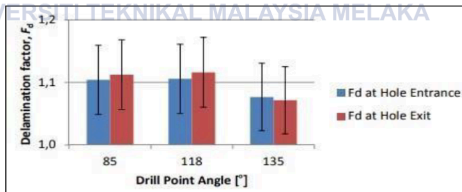
Figure 2.21: Drilling of 0.02 mm/rev of feed rate (Maoinsir et al., 2014)
