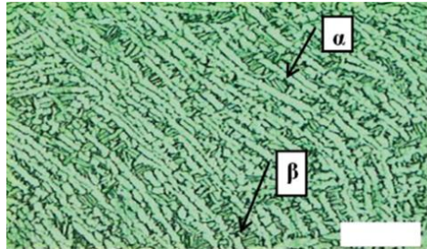
Figure 1: Microstructure of Ti-6Al-4V ELI.
