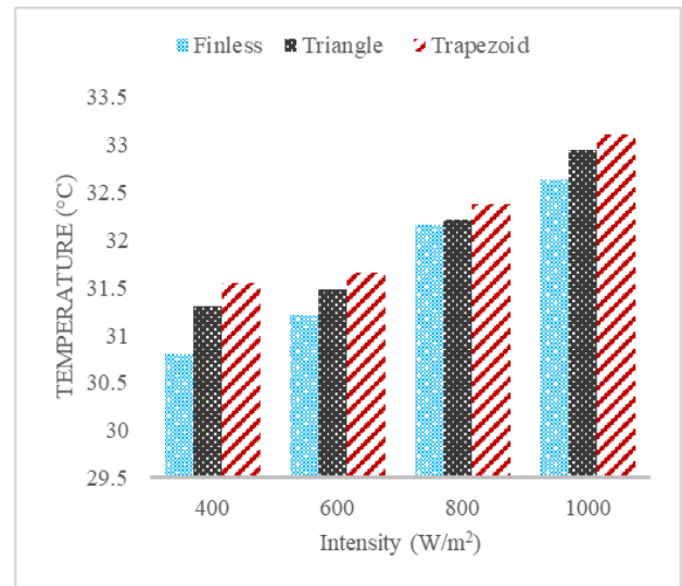
Figure 11. Mean temperature distribution in the PVT system
