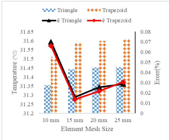
Figure 7. Mesh independence test
