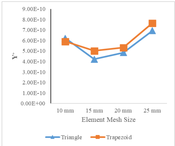
Figure 8. Effect of mesh element size on average Y^+ distribution in the PCM domain
