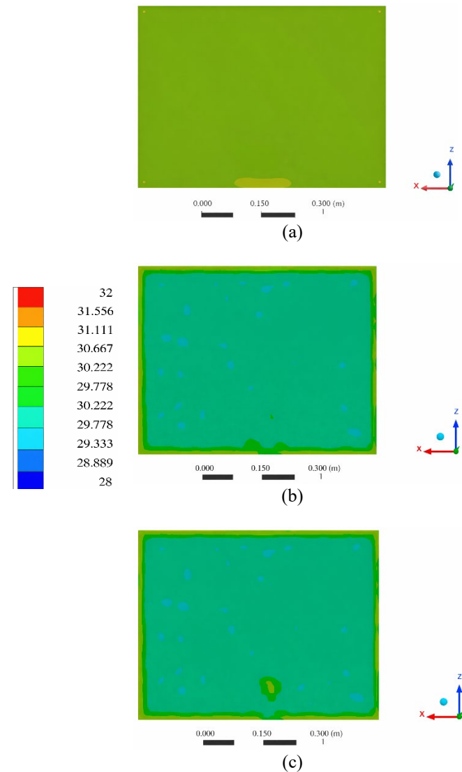
Figure 9. PV temperature distribution (a) Finless (b) Triangle (c) Trapezoid
