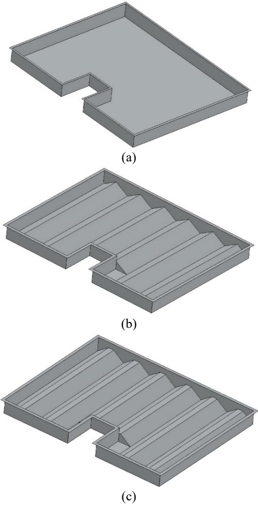
Figure 3. Model of the fin container (a) Finless (b) Triangle (c) Trapezoid
