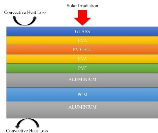
Figure 2. Illustration of the Photovoltaic Thermal–Phase Change Material system
