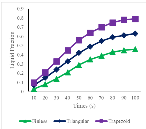
Figure 10. Temporal evolution of the melting liquid fraction at 1000 W/m 2
