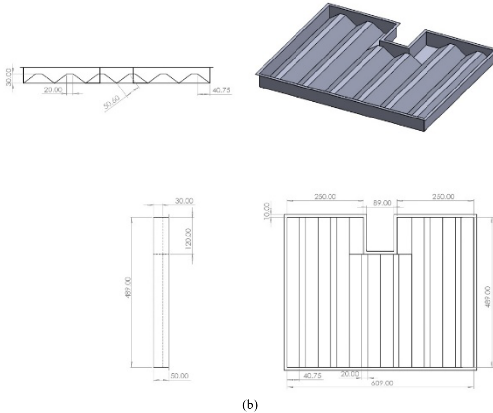
Figure 4. Detail geometry fin container of the (a) Triangle (b) Trapezoid
