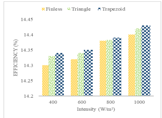
Figure 13. Electrical efficiency performance of PVT system
