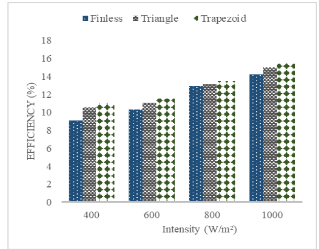
Figure 12. Thermal efficiency performance of PVT system
