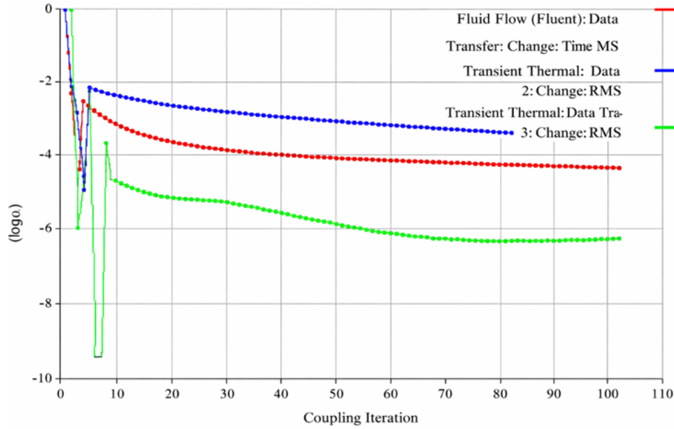
Figure 5. Convergence curve of iterations over simulation time
