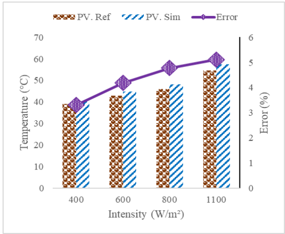
Figure 6. Validation based on established study [41]
