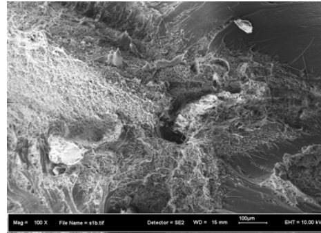
Fig.3a. Magnification at Mixture of 90 wt. % LDPE & 10 wt. % wax.
