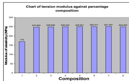
Fig.1b. Chart of tension modulus against percentage composition of LDPE, wax & coconut coir.
