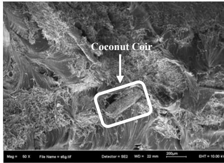
Fig.5a. Magnification at Mixture of 90 wt. % LDPE, 4 wt. % wax & 6 wt. % coconut coir.
