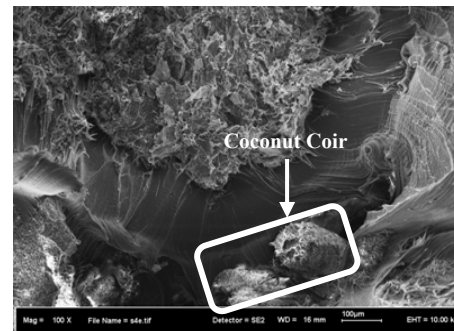
Fig.4b. Magnification at Mixture of 90 wt. % LDPE, 5 wt. % wax & 5 wt. % coconut coir.
