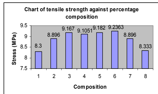
Fig.1a. Chart of tensile strength against percentage composition of LDPE, wax & coconut coir.
