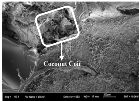
Fig.5b. Magnification at Mixture of 90 wt. % LDPE, 10 wt. % coconut coir.
