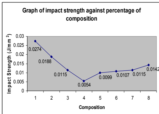
Fig.2b. Graph of Impact Strength against percentage composition of LDPE, wax & coconut coir
