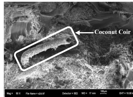
Fig.3b. Magnification at Mixture of 90 wt. % LDPE, 8 wt. % wax & 2 wt. % coconut coir
