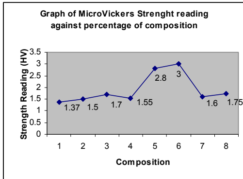
Fig.2a. Graph of Microvickers strength against percentage composition of LDPE, wax & coconut coir
