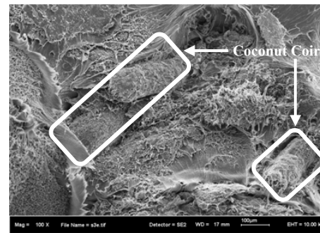
Fig.4a. Magnification at Mixture of 90 wt. % LDPE, 6 wt. % wax & 4 wt. % coconut coir
