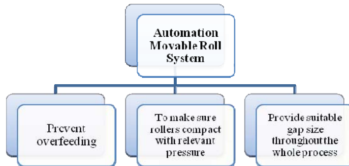
Figure 3. Functional decomposition of automation movable roll system
