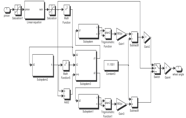
Figure 3. Propose rack and pinion steering system modeled in MATLAB
