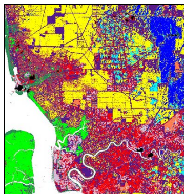
Fig. 2. ML classification using band 1, 2, 3, 4, 5 and 7 of Landsat TM and the class areas in terms of square kilometre and percentage.
