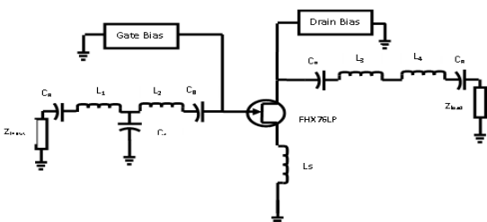
Figure 5: The Schematic Circuit for Single LNA
