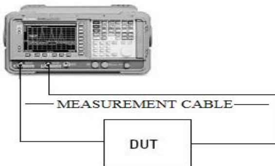
Figure 7: Setup for device under test S Measurement using Network Analyzer
