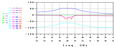
Figure 6c: S-parameters for cascode and cascaded
