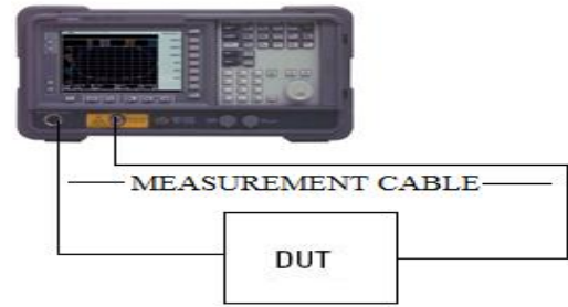
Figure 9: Measurement setup for device under test for Noise Figure
