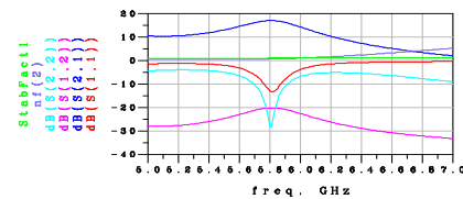
Figure 6a: S-parameters for Cascode
