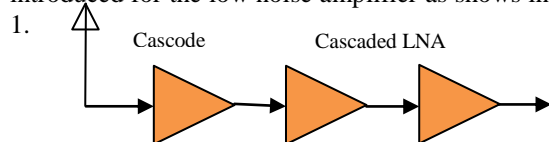
Figure 1: Cascode and Cascaded LNA
