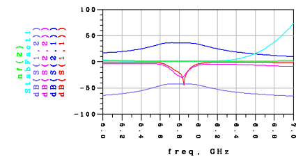
Figure 6b: S-parameters for cascaded
