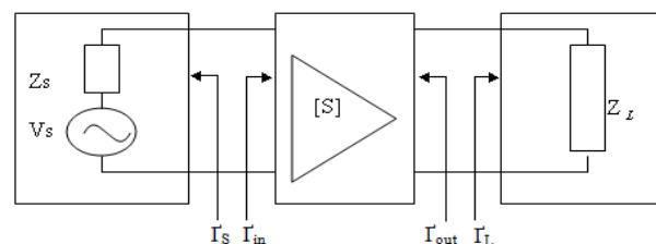
Figure 3: I/O circuit of 2-port network
