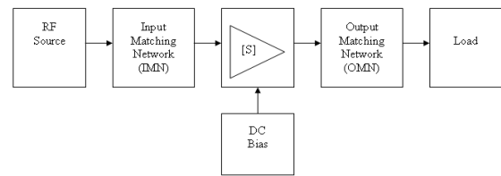
Figure 2: Typical amplifier design
