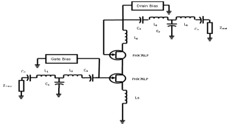
Figure 4: The Schematic Circuit for Cascode LNA
