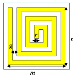
Figure 1: Schematic diagram for single unit of spiral split ring resonator. Dimension: m and n = 2.6 mm, r = 0.2 mm, g = 0.2 mm, thickness of copper = 0.035 mm, FR4 substrate thickness = 1.6 mm.
