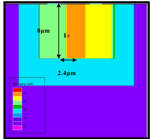
Figure 4: Intrinsic with 2.4\mu\text{m} \times 8\mu\text{m}
