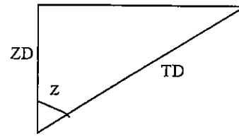
Fig. 1 Illustration for obliquity factor (mapping function) between zenith and slant direction
