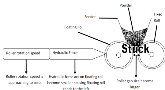
Fig. 2. General concept design draft of automation movable roll system
