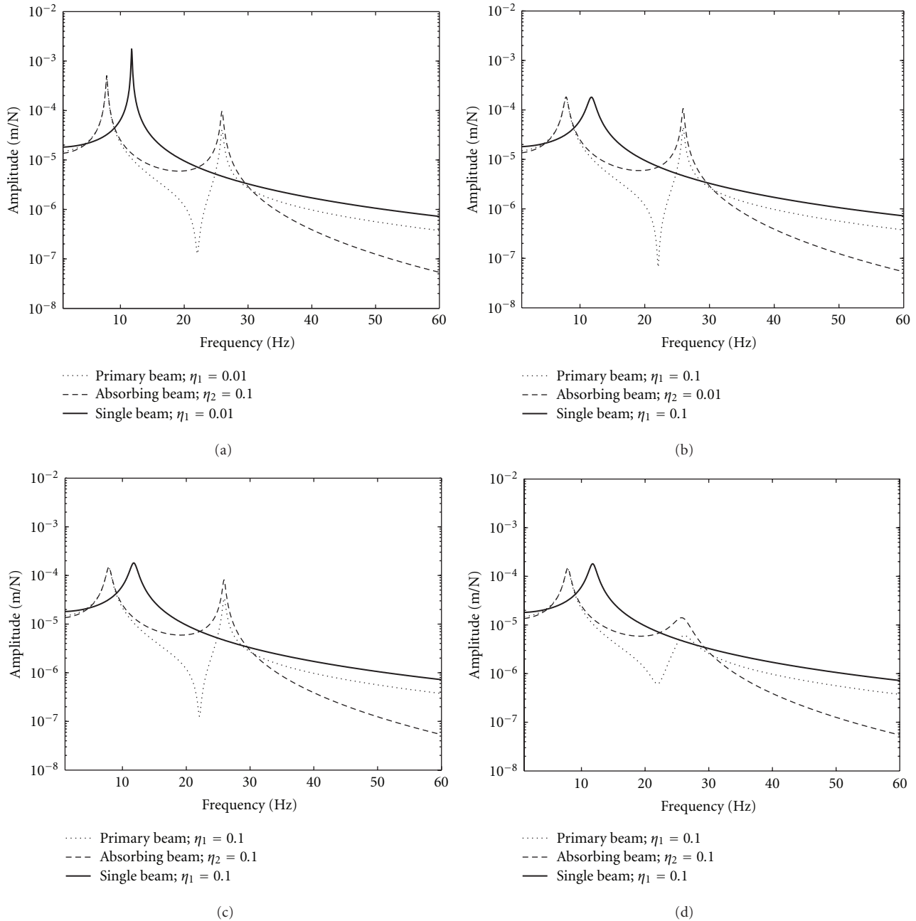
FIGURE 5: Effect of structural damping of the beam on the vibration amplitude at the midspan location of the double-beam system ( e = 0.25 , \mu = 0.4 ): (a)–(c) \zeta = 0.01 and (d) \zeta = 0.1 .
