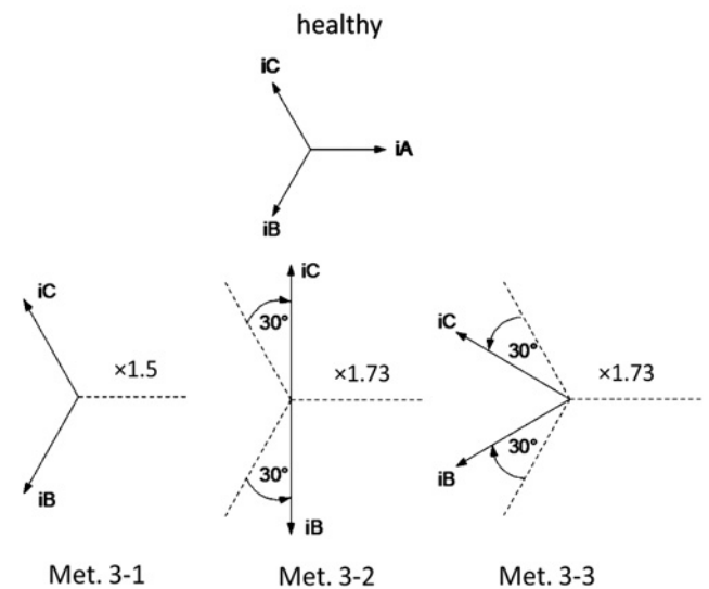
Figure 6 Current diagrams for healthy and various FT strategies for a three-phase machine
