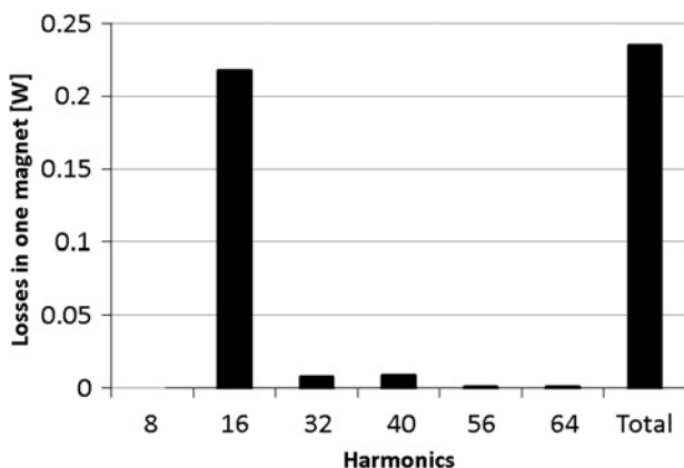
Figure 14 Machine 3b: losses owing to each space harmonics in one magnet when one phase is lost and FT strategy with current shifting is used (Method 3-3)
